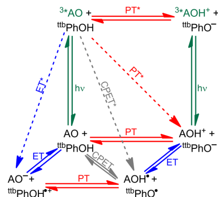
Scheme 1. PCET Square Scheme Incorporating Ground- and Excited-State Reactivity
